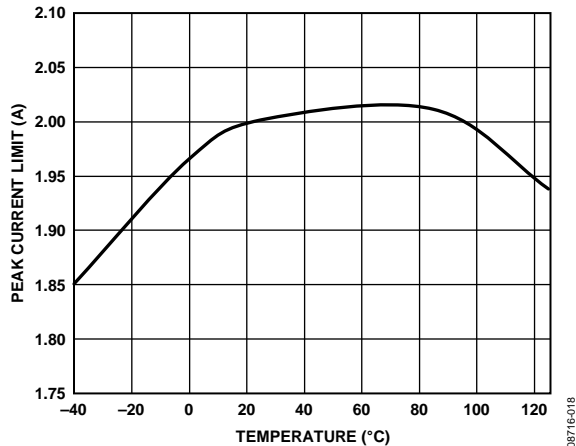
Figure 18. Peak Current Limit vs. Temperature (ADP2120, V_{IN} = 3.3 V )
