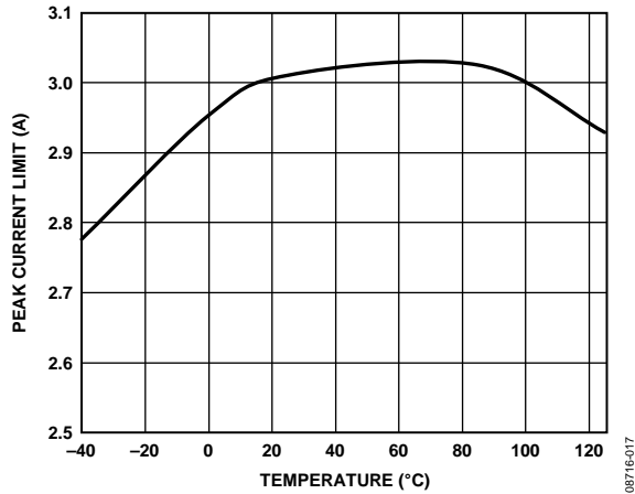
Figure 17. Peak Current Limit vs. Temperature (ADP2119, V_{IN} = 3.3 V )
