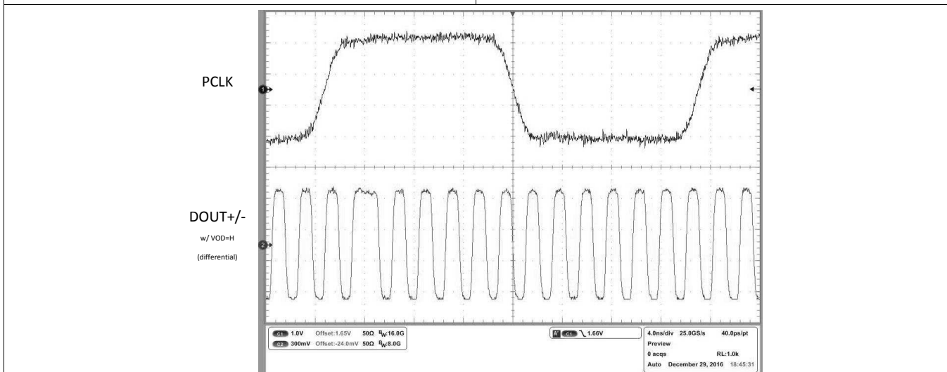
Figure 30. Input PCLK = 33 MHz and Associated DOUT Serial Stream With VODSEL = H
