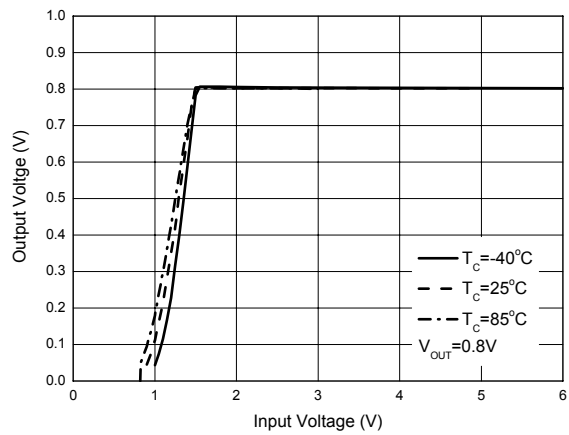
Figure 27. Output Voltage vs. Input Voltage (I OUT =300mA)
