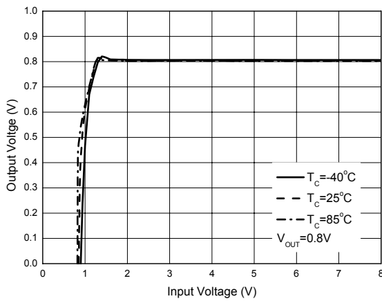
Figure 26. Output Voltage vs. Input Voltage (I OUT =0mA)
