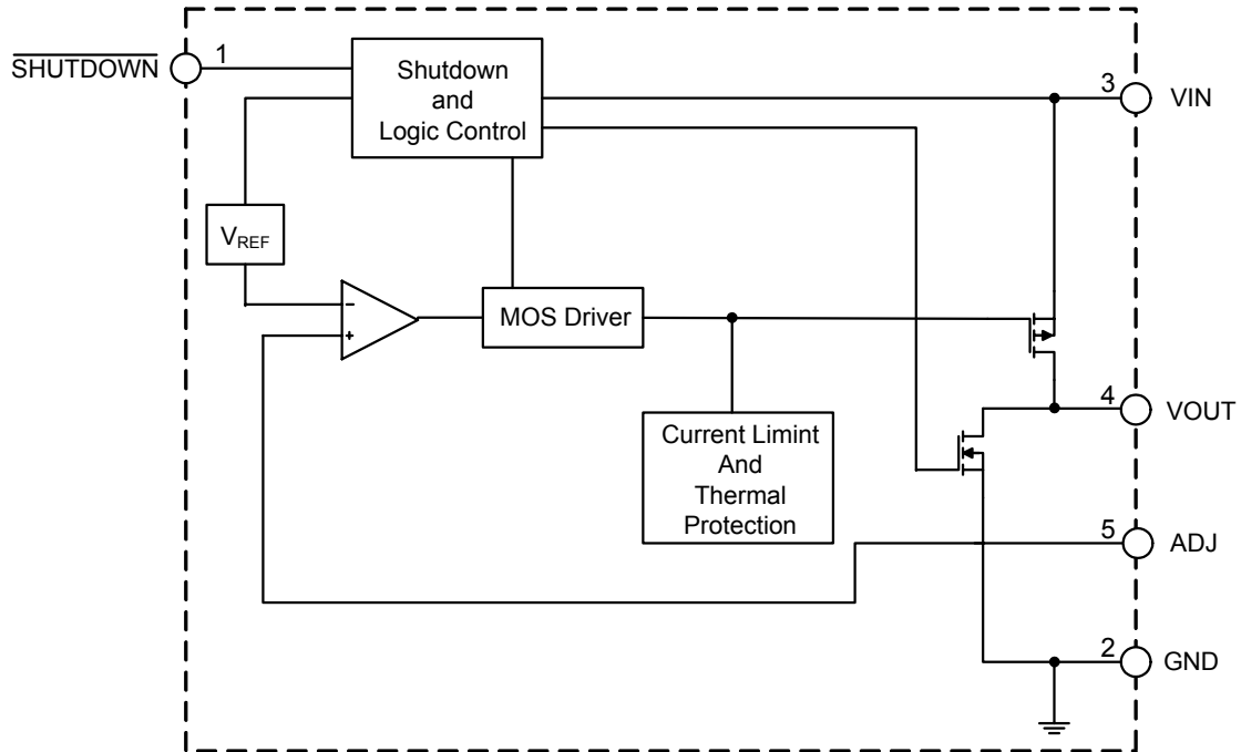
Adjustable Version
