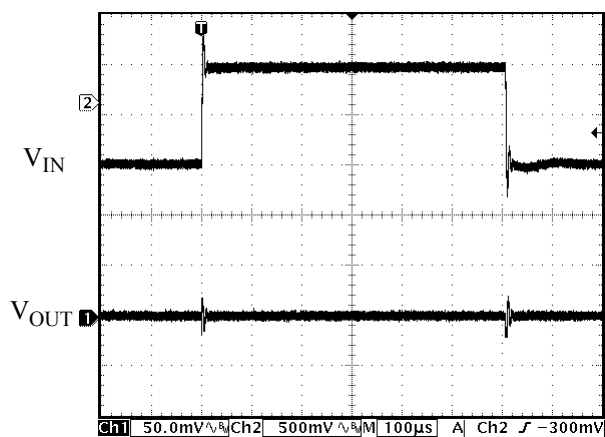
Figure 33. Line Transient
