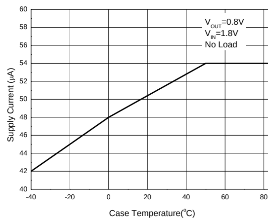
Supply Current vs. Case Temperature
