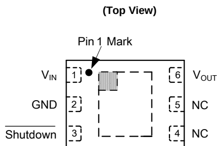
DFN-1.5x2-6
