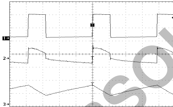
Figure 39. NCP1402SN19T1 Operating Waveforms (Medium Load)
