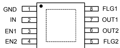
MSOP-8EP
