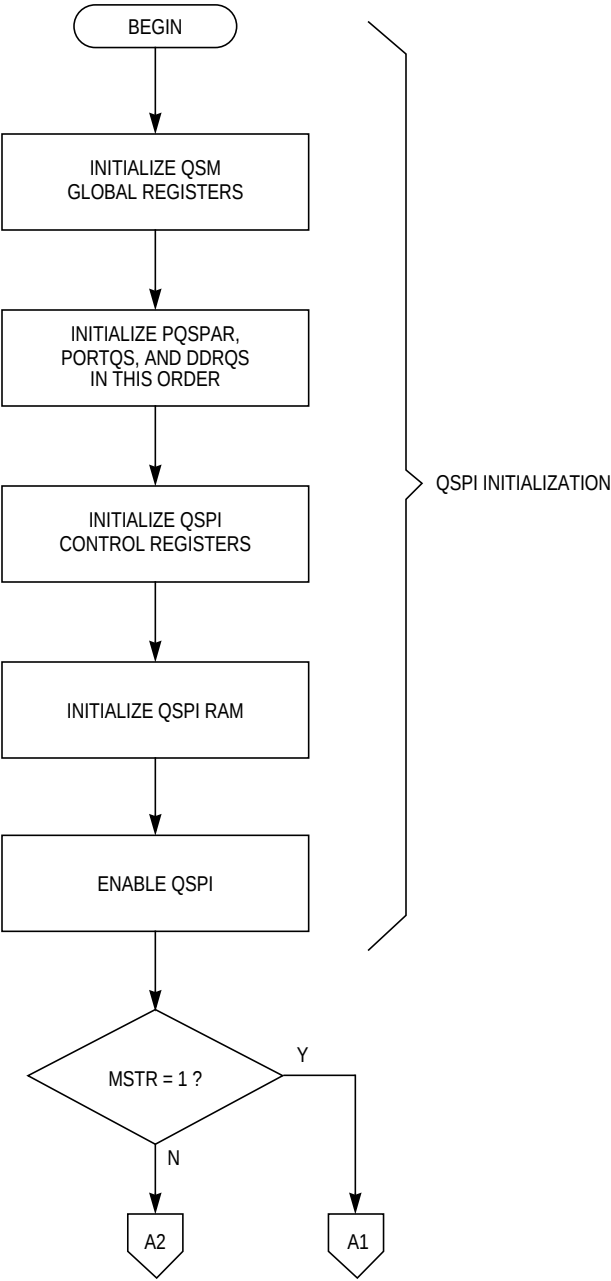
Figure 9-4 Flowchart of QSPI Initialization Operation
