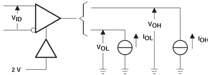
Figure 6-1. V_{OH} and V_{OL} Test Circuit
