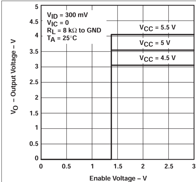
Figure 5-1. Output Voltage vs Enable Voltage
