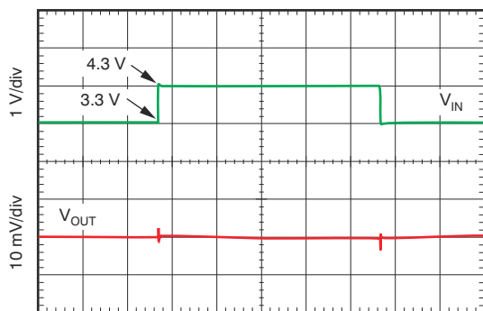
Figure 6-21. Line Transient Response
