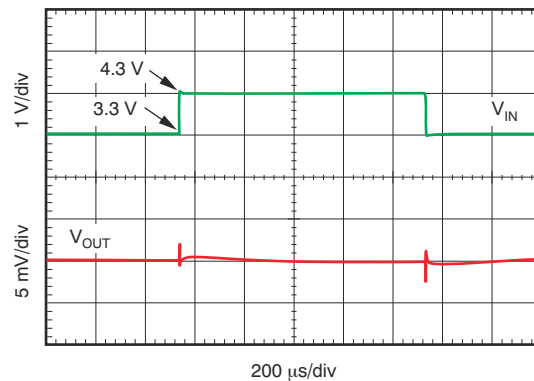
Figure 8-3. Line Transient Response V_{OUT} = 1.8\ \text{V} , I_{OUT} = 500\ \text{mA}
