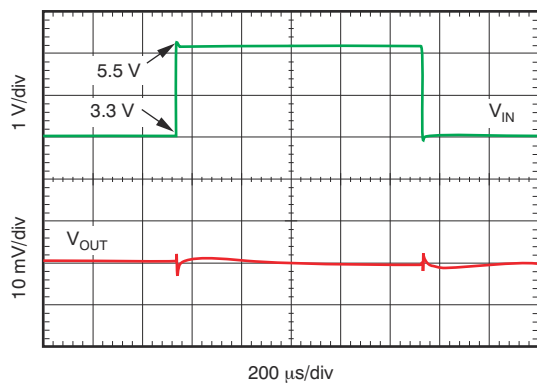
Figure 6-25. Line Transient Response
