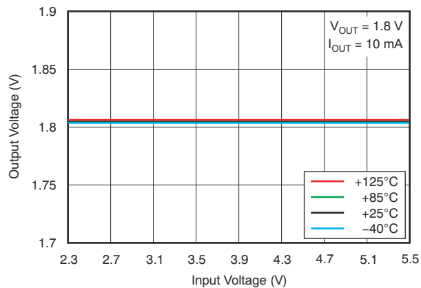
Figure 6-1. Line Regulation
