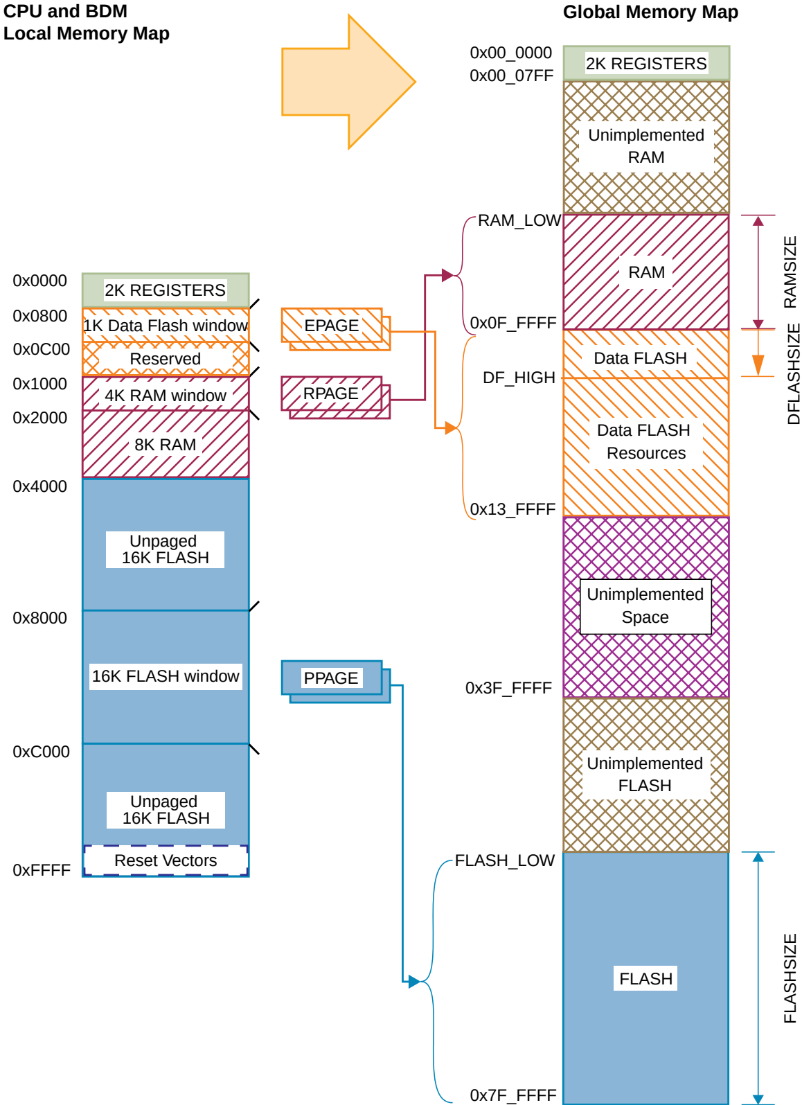
Figure 3-19. S12X CPU & BDM Global Address Mapping
