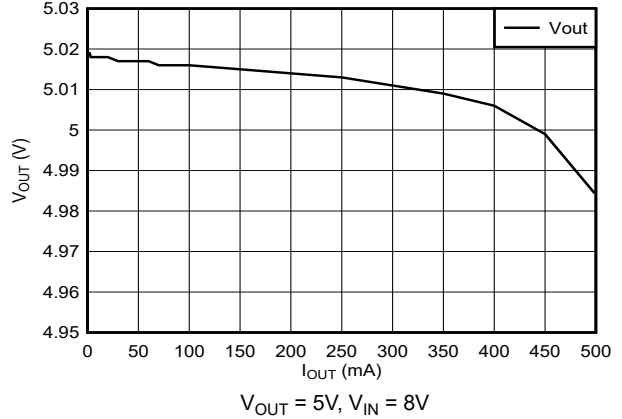
Figure 5-2. Load Regulation at T_J = 25^\circ C (New Chip)
