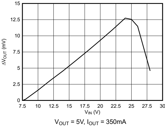
Figure 5-3. Line Regulation at T_J = 25^\circ C (New Chip)
