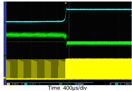
Short Circuit Recovery ( V_{IN}=12\text{V} , V_{OUT}=3.3\text{V} , I_{OUT}=3\text{A} )
