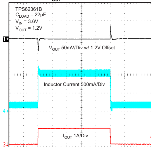
LOAD TRANSIENT RESPONSE I_{OUT} RANGE: 200mA to 1A
