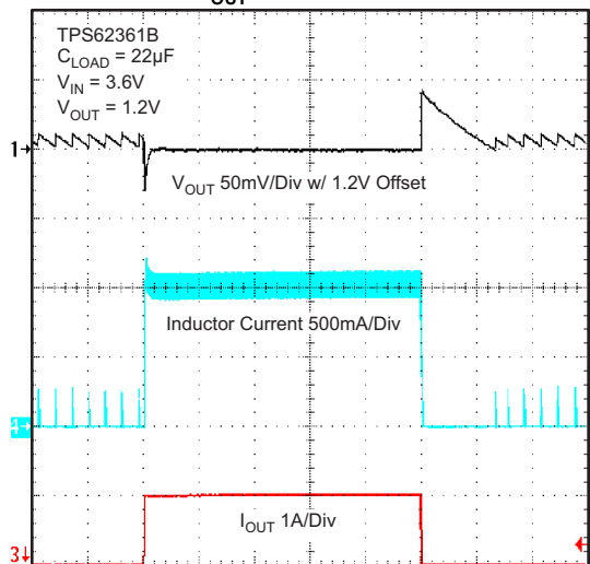
LOAD TRANSIENT RESPONSE I_{OUT} RANGE: 5mA to 1A
