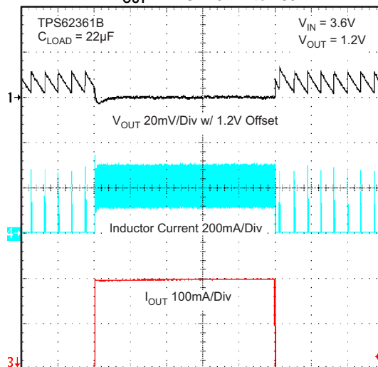
LOAD TRANSIENT RESPONSE I_{OUT} RANGE: 5mA to 200mA
