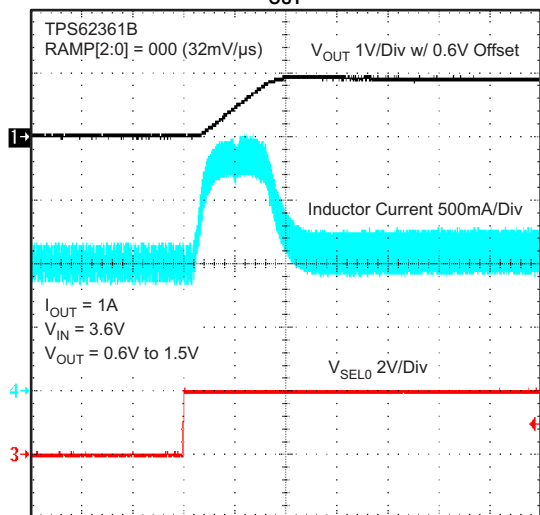
OUTPUT VOLTAGE RAMP CONTROL I_{OUT} = 1A
