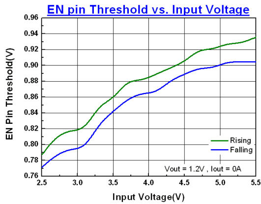
Figure 20. EN Pin Threshold vs. Input Voltage
