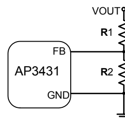
Figure 34. Setting the Output Voltage
