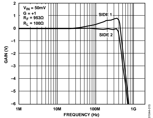
Figure 16. Gain vs. Frequency Response, G = +1 (See Figure 42)
