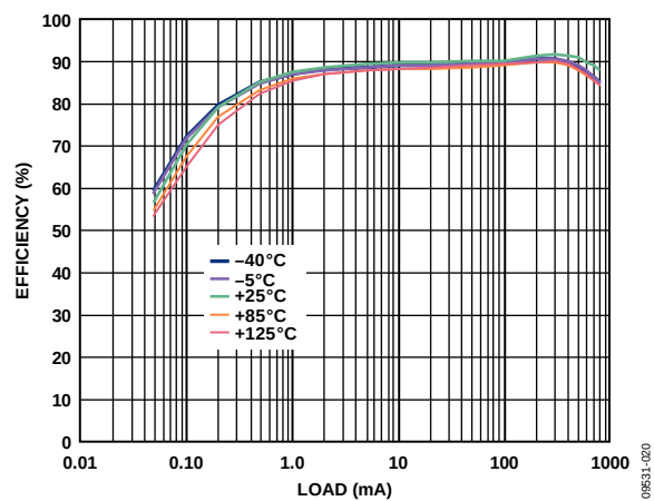
Figure 20. Efficiency vs. Load Current, V_{OUT} = 3.3\text{ V} , Different Temperatures, V_{IN} = 7.3\text{ V}
