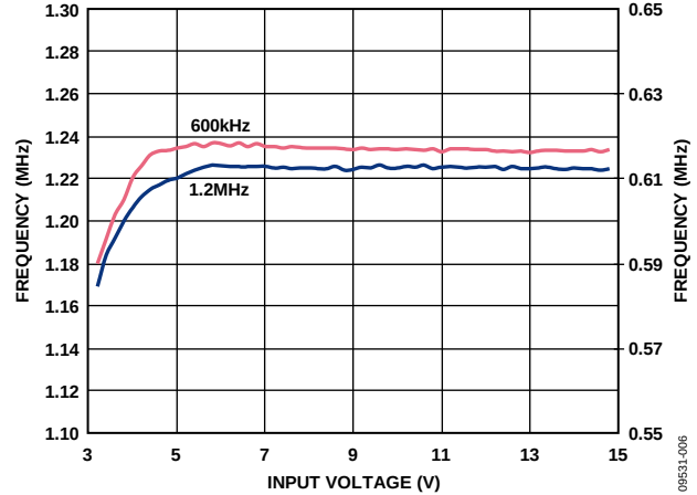
Figure 6. Switching Frequency vs. Input Voltage, FPWM Mode
