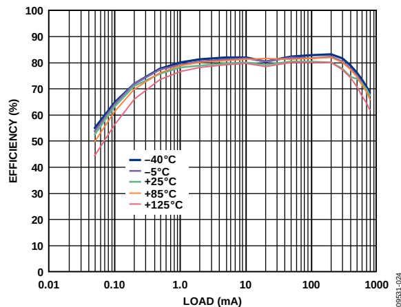
Figure 24. Efficiency vs. Load Current, V_{OUT} = 1.2\text{ V} , Different Temperatures, V_{IN} = 4\text{ V}
