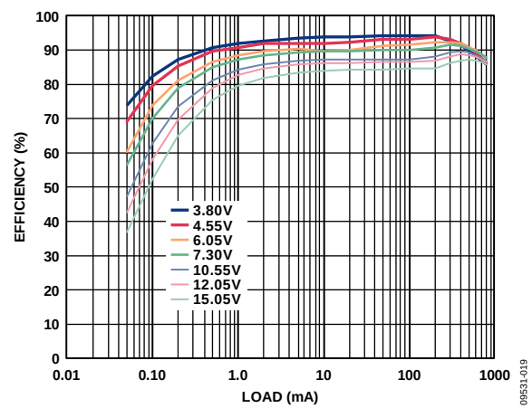
Figure 19. Efficiency vs. Load Current, V_{OUT} = 3.3\text{ V} , Different Input Voltages
