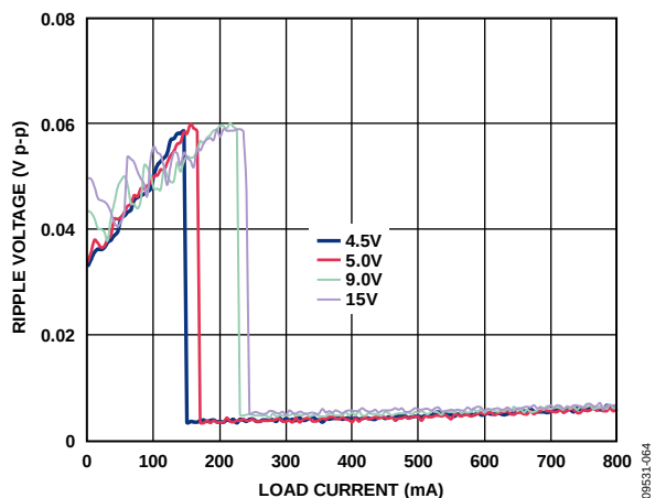
Figure 64. Output Ripple vs. Load Current, V_{OUT} = 3.3 V, Different Input Voltages, Automatic Mode
