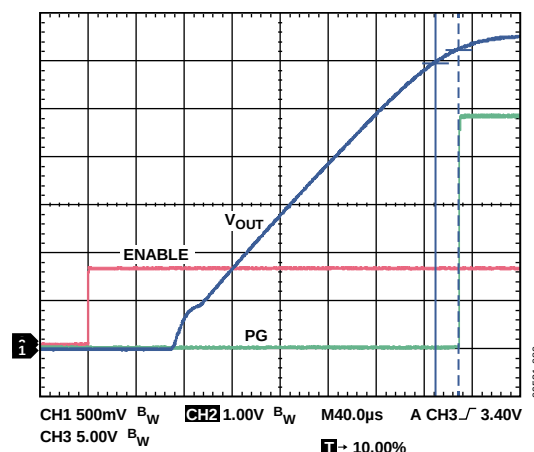
Figure 80. Typical PG Timing at Startup
