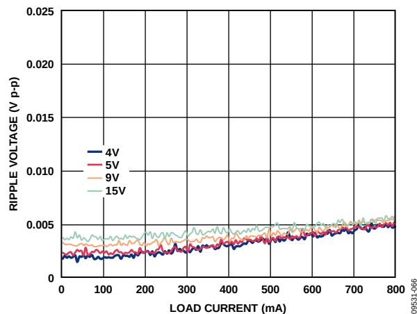
Figure 66. Output Ripple vs. Load Current, V_{OUT} = 3.3 V, Different Input Voltages, Force PWM Mode
