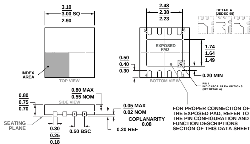
Figure 93. 8-Lead Lead Frame Chip Scale Package [LFCSP] 3 mm × 3 mm Body and 0.75 mm Package Height (CP-8-5)
