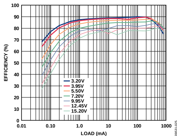
Figure 25. Efficiency vs. Load Current, V_{OUT} = 1.8\text{ V} , Different Input Voltages
