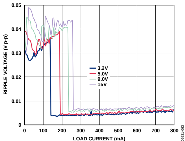
Figure 63. Output Ripple vs. Load Current, V_{OUT} = 1.8 V, Different Input Voltages, Automatic Mode
