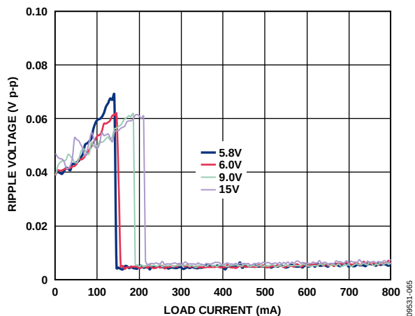
Figure 65. Output Ripple vs. Load Current, V_{OUT} = 5 V, Different Input Voltages, Automatic Mode
