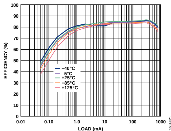
Figure 26. Efficiency vs. Load Current, V_{OUT} = 1.8\text{ V} , Different Temperatures, V_{IN} = 4\text{ V}
