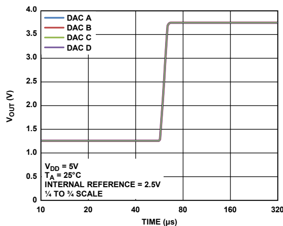
Figure 37. Settling Time, 5.25 V
