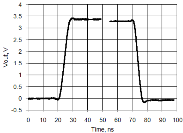
Figure 11-16. USBIO Output Rise and Fall Times, GPIO Mode, V_{\text{DD}} = 3.3\text{ V} , 25 pF Load
