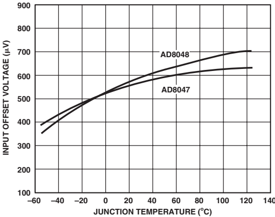
TPC 48. AD8047/AD8048 Input Offset Voltage vs. Temperature
