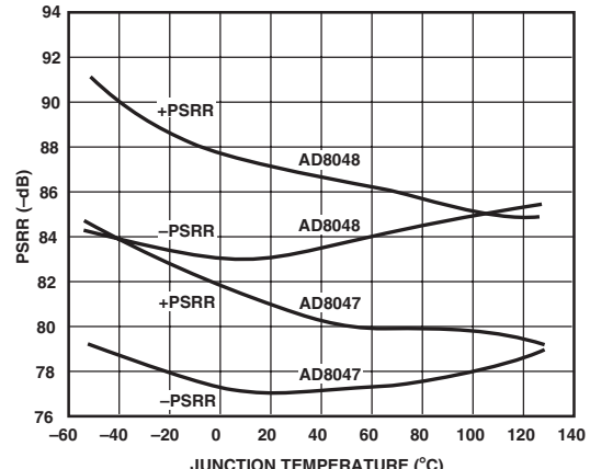
TPC 45. AD8047/AD8048 PSRR vs. Temperature
