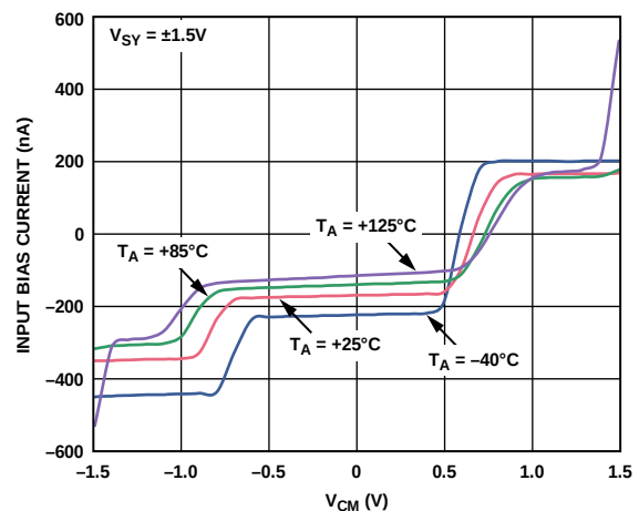
Figure 20. Input Bias Current vs. V_{CM} for Various Temperatures
