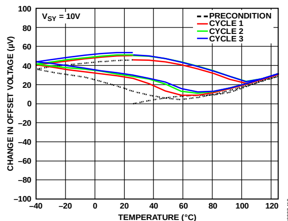
Figure 113. Change in Offset Voltage over Three Full Temperature Cycles
