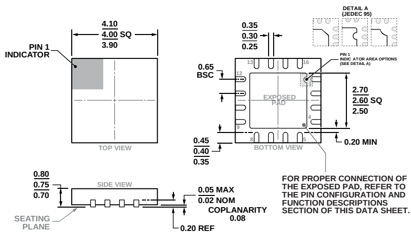
Figure 119. 16-Lead Lead Frame Chip Scale Package [LFCS] 4 mm × 4 mm Body and 0.75 mm Package Height (CP-16-17)
