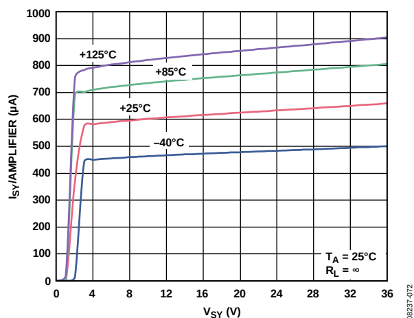
Figure 103. Supply Current ( I_S ) per Amplifier vs. Supply Voltage ( V_S ) for Various Temperatures
