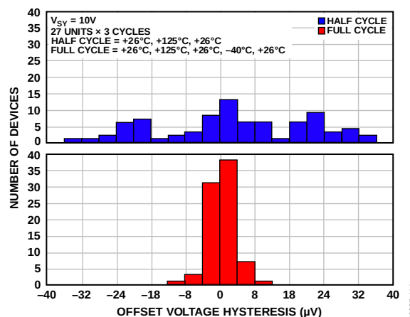
Figure 114. Histogram Showing the Temperature Hysteresis of the Offset Voltage over Three Full Cycles and over Three Half Cycles
