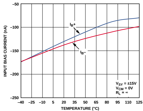
Figure 81. Input Bias Current vs. Temperature
