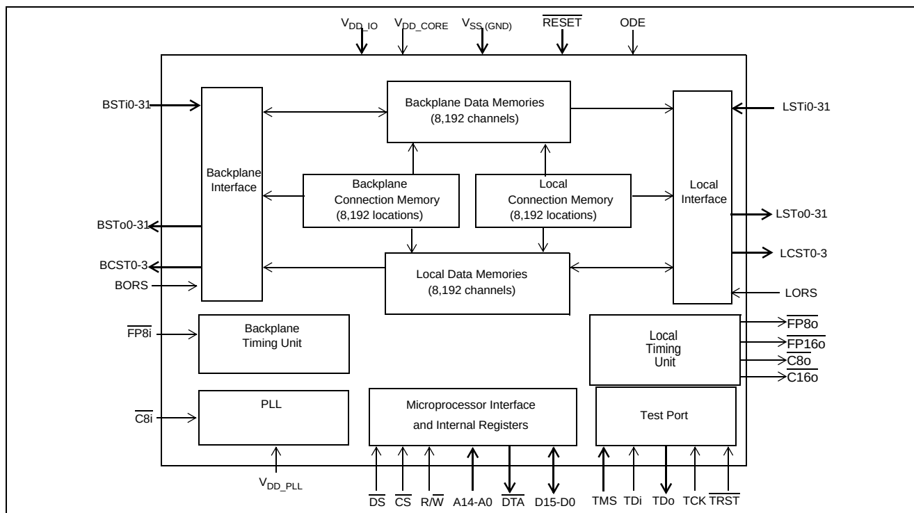
Figure 1 - MT90869 Functional Block Diagram
