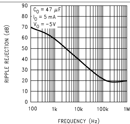
Figure 8. Ripple Rejection
