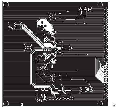
Figure 51. Bottom Routing
