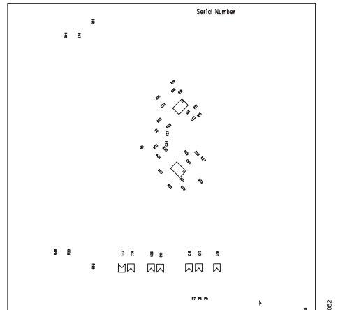
Figure 52. Bottom Silkscreen
