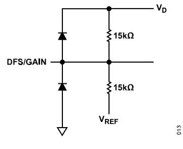
Figure 13. DFS/Gain Input
