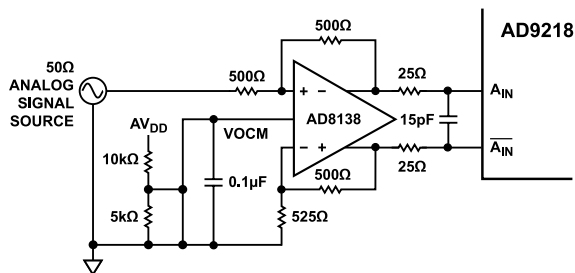
Figure 43. Using the AD8138 to Drive the AD9218
