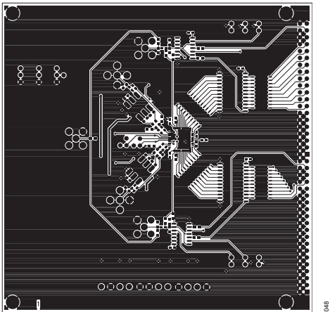
Figure 48. Top Routing
