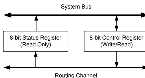
Figure 7-10. Status and Control Registers
