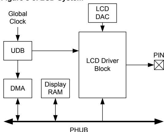
Figure 8-9. LCD System
