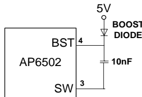
Figure 4—External Bootstrap Compensation Components
