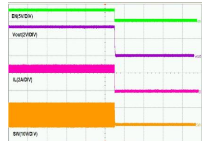
Time -5ms/div
