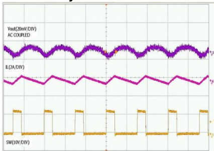
Time -2µs/div
