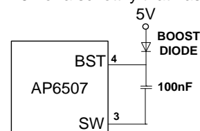
Figure 3. External Bootstrap Diode
