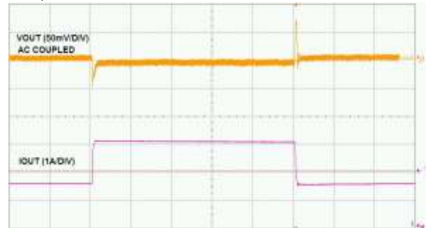
Time- 200 \mu s/div Load Transient Test I_{OUT} = 1.5A to 3A . Step at 0.8A/\mu
