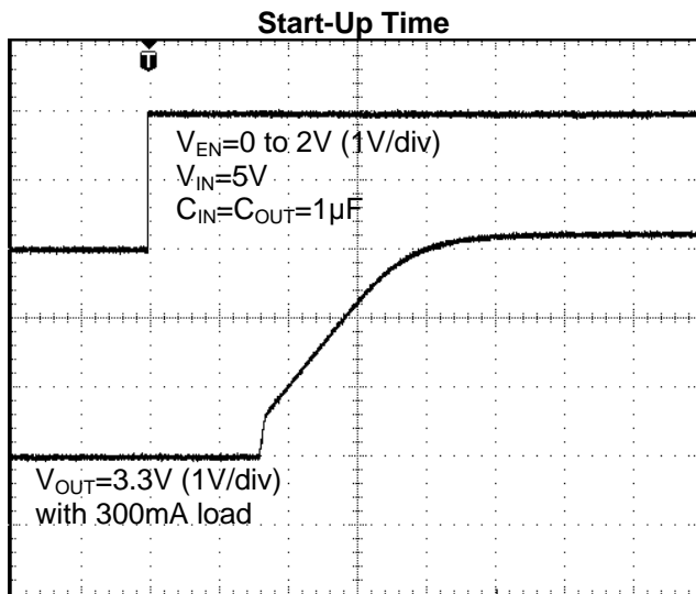
Time (40µs/div)
