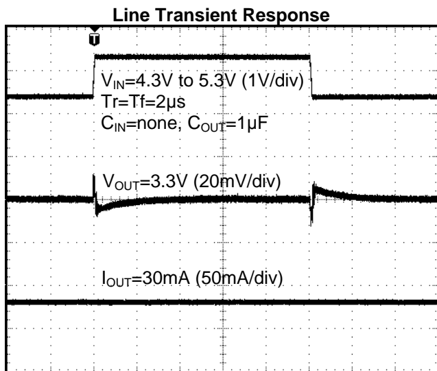
Time (40µs/div)
