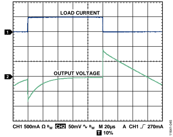
Figure 51. Load Transient Response, C_{IN} = C_{OUT} = 1\text{ }\mu\text{F} , I_{LOAD} = 1\text{ mA} to 500\text{ mA} , V_{OUT} = 1.8\text{ V} , V_{IN} = 5\text{ V}
