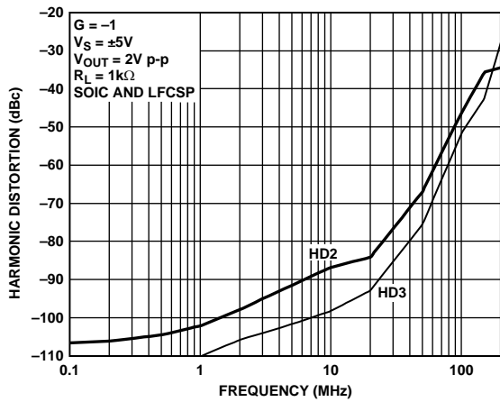
Figure 20. Harmonic Distortion vs. Frequency for Various Packages
