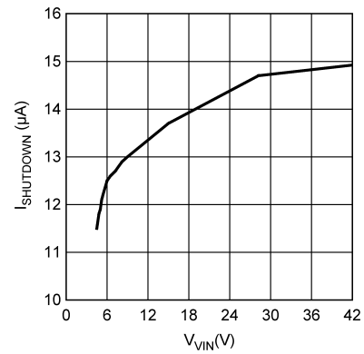
Figure 6-4. Shutdown Current
