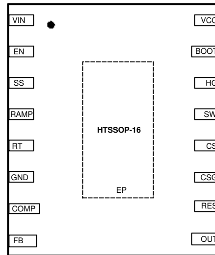
Figure 5-2. LM25088-2 16-Pin PWP Package (Restart Version) (Top View)
