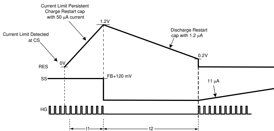
Figure 7-8. Current Limit Restart Timing Diagram
