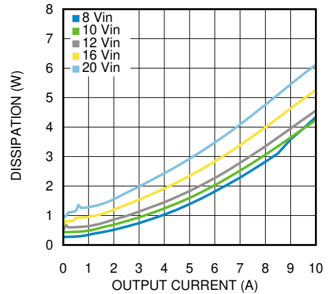
Figure 6-2. Dissipation 5-V Output at 25°C
