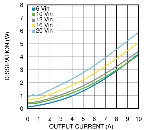
Figure 6-4. Dissipation 3.3-V Output at 25°C
