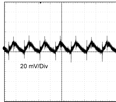
Figure 6-36. Output Ripple
