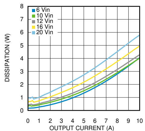
Figure 6-6. Dissipation 2.5-V Output at 25°C
