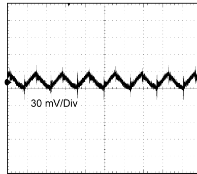
Figure 6-34. Output Ripple
