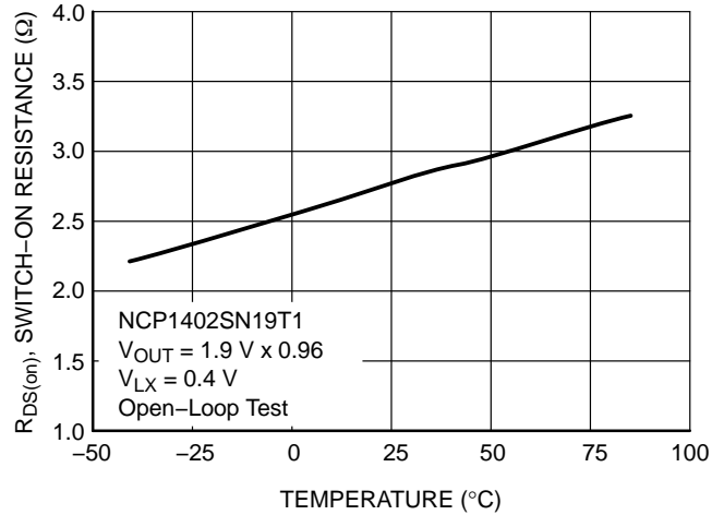
Figure 30. NCP1402SN19T1 Switch-on Resistance vs. Temperature
