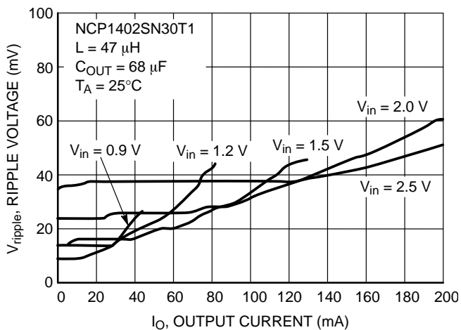
Figure 52. NCP1402SN30T1 Ripple Voltage vs. Output Current
