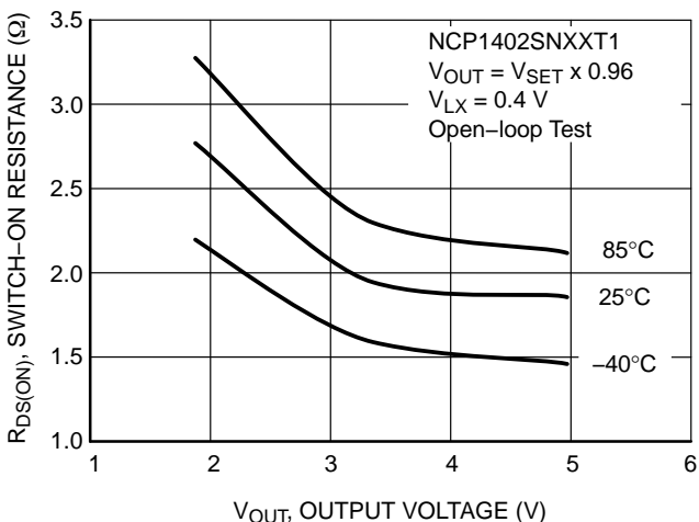
Figure 56. NCP1402SNXXT1 Switch-On Resistance vs. Output Voltage
