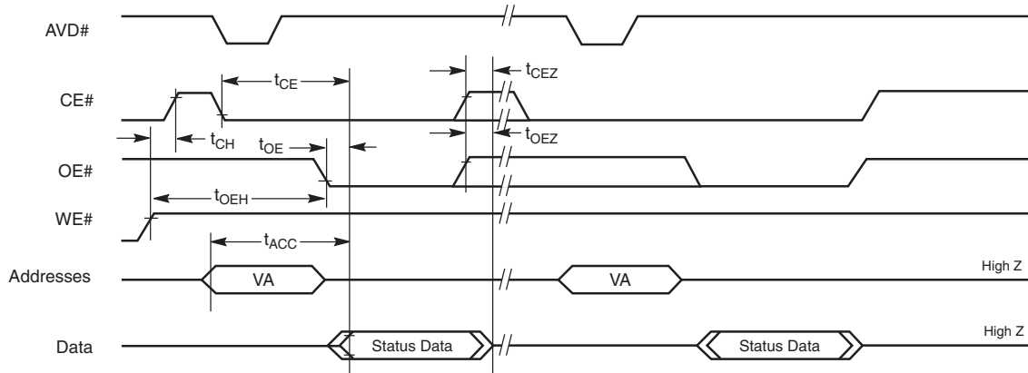
Figure 11.19 Data# Polling Timings (During Embedded Algorithm)
