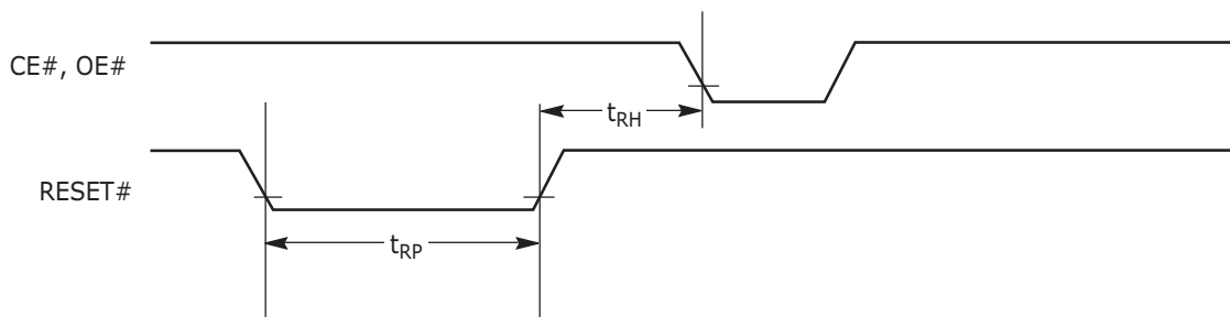
Figure 11.14 Reset Timings
