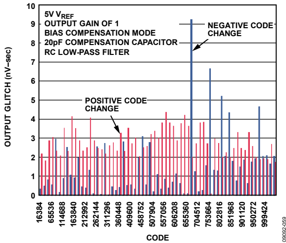
Figure 42. 6 MSB Segment Glitch Energy for ±10V VREF
