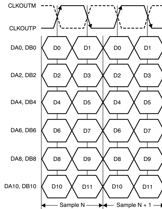
Figure 4. ADS4226/25/22 LVDS Interface Timing Diagram
