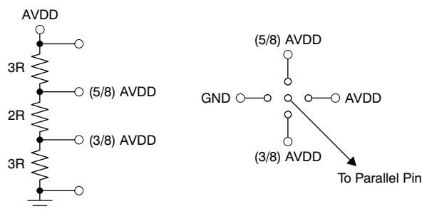
Figure 150. Simple Scheme to Configure the Parallel Pins
