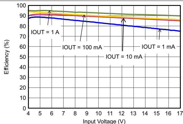
Figure 13. Efficiency With 2.5 MHz
