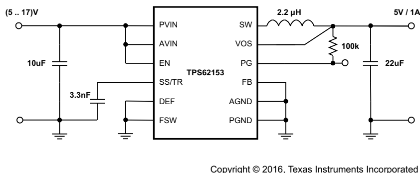
Figure 47. 5-V, 1-A Power Supply
