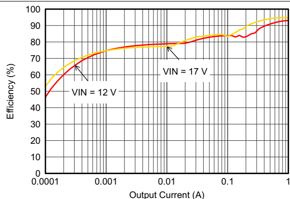
Figure 10. Efficiency With 1.25 MHz
