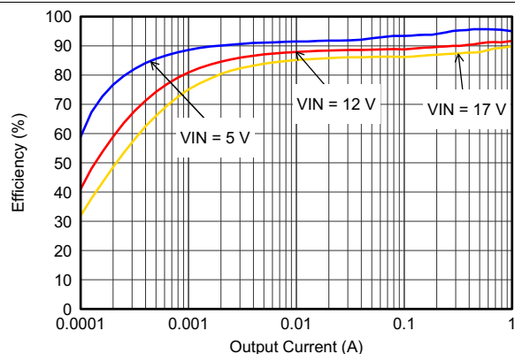
Figure 12. Efficiency With 2.5 MHz
