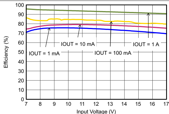
Figure 11. Efficiency With 1.25 MHz
