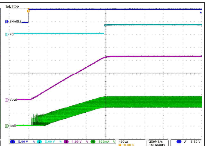
Figure 41. Start-Up Into 1 A
