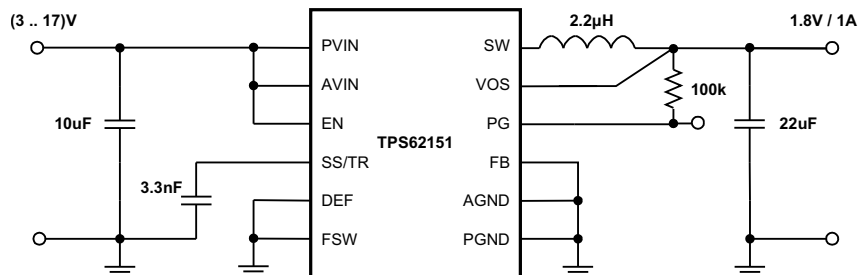
Figure 50. 1.8-V, 1-A Power Supply
