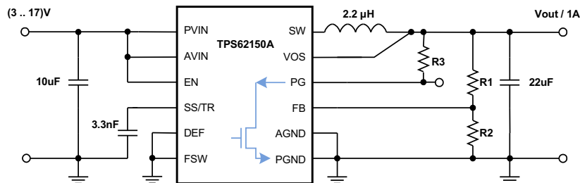
Figure 45. Discharge V_{OUT} Through PG Pin with TPS62150A
