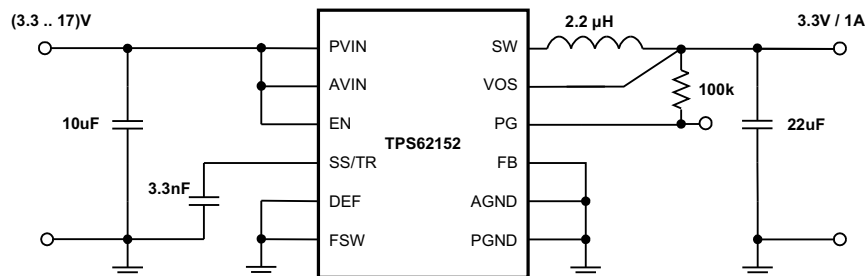
Figure 48. 3.3-V, 1-A Power Supply
