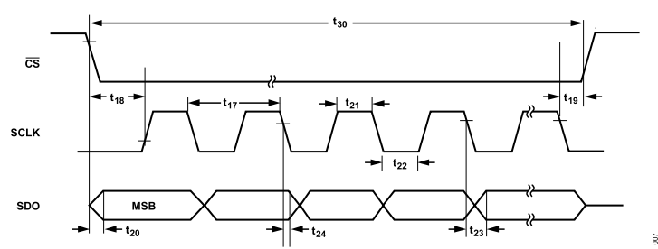
Figure 7. SPI Serial Read Timing Diagram
