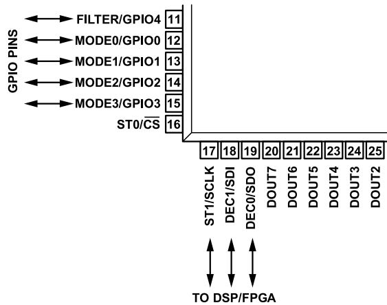
Figure 113. AD7768 GPIO Functionality
