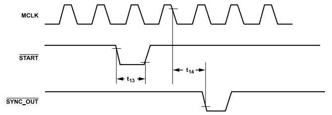
Figure 5. Asynchronous START and SYNC_OUT Timing Diagram
