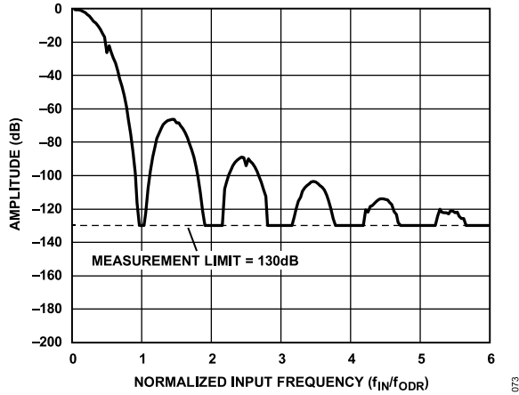
Figure 60. Amplitude vs. Normalized Input Frequency ( f_{IN}/f_{ODR} ), Sinc5 Filter Profile
