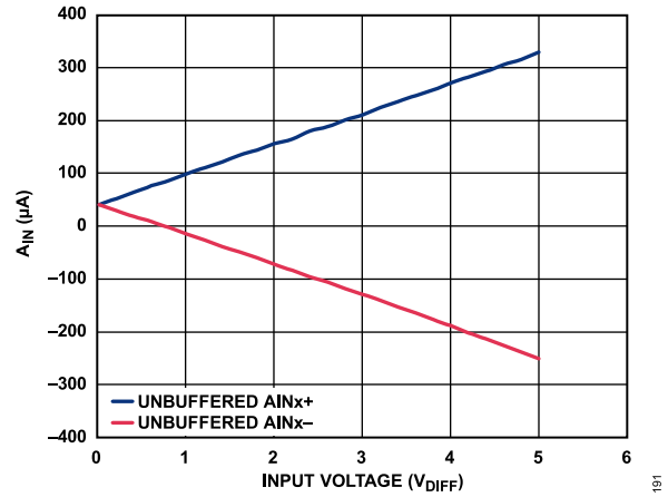
Figure 85. Analog Input Current ( I_{AIN} ) vs. Input Voltage, Analog Input Precharge Buffer Off, V_{CM} = 2.5\text{ V} , f_{MOD} = 8.192\text{ MHz}
