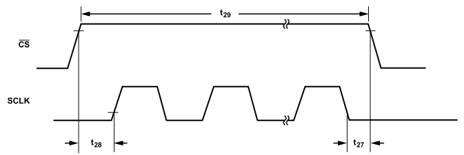
Figure 9. SCLK Enable and Disable Timing Diagram
