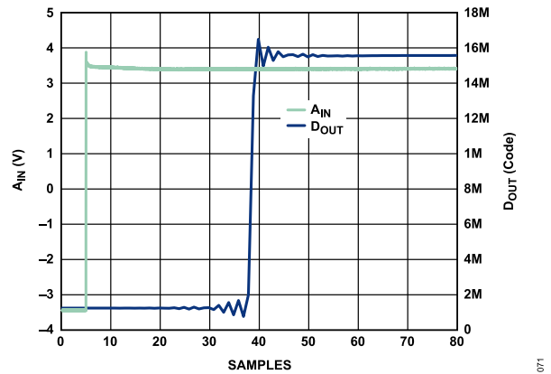
Figure 58. Step Response, Wideband Filter
