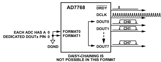
Figure 95. AD7768 FORMATx = 00, Eight Data Output Pins
