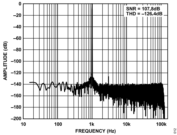
Figure 12. Fast Fourier Transform (FFT), Fast Mode, Wideband Filter, -0.5 dBFS
