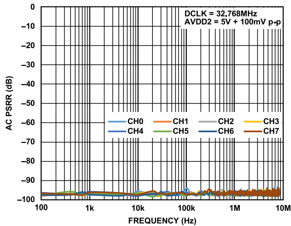
Figure 55. AC PSRR vs. Frequency, AVDD2
