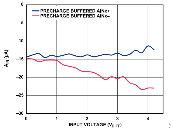
Figure 86. Analog Input Current ( I_{AIN} ) vs. Input Voltage, Analog Input Precharge Buffer On, V_{CM} = 2.5\text{ V} , f_{MOD} = 8.192\text{ MHz}
