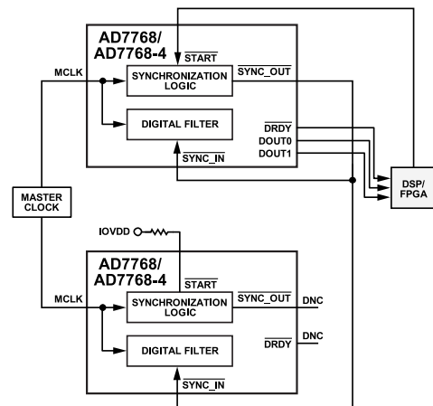
Figure 110. Synchronizing Multiple AD7768/AD7768-4 Devices Using \overline{\text{SYNC\_OUT}}
