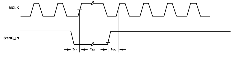
Figure 6. Synchronous SYNC_IN Pulse Timing Diagram
