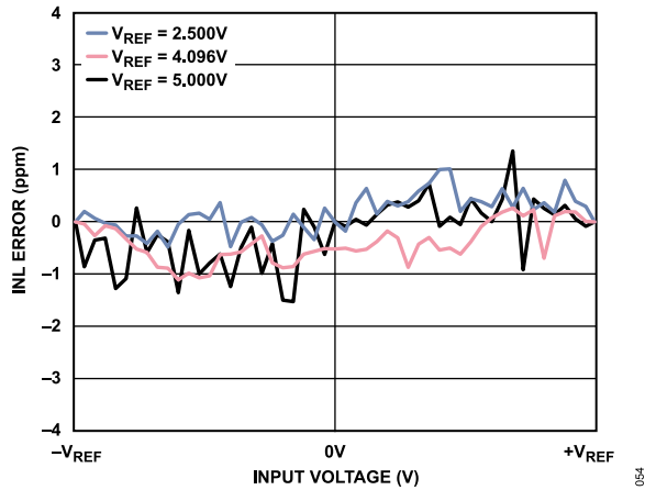
Figure 42. INL Error vs. Input Voltage for Various V REF Levels, Low Power Mode
