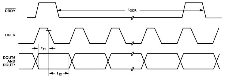
Figure 4. Daisy-Chain Setup and Hold Timing Diagram
