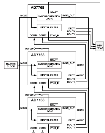
Figure 109. Daisy-Chaining Multiple AD7768 Devices
