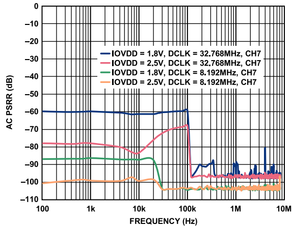
Figure 56. AC PSRR vs. Frequency, IOVDD
