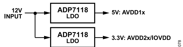
Figure 74. Power Supply Configuration
