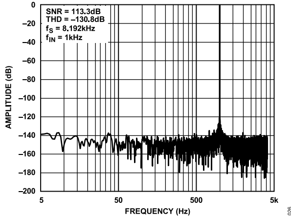
Figure 24. FFT One Shot Mode, Sinc5 Filter, Median Mode, Decimation = x64, -0.5 dBFS, SYNC_IN Frequency = MCLK/4000
