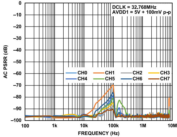
Figure 54. AC PSRR vs. Frequency, AVDD1
