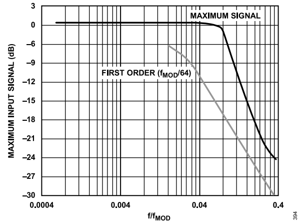
Figure 94. Maximum Input Signal vs. Frequency
