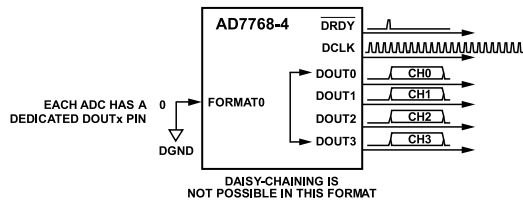
Figure 97. AD7768-4 FORMAT0 = 0, Four Data Output Pins
