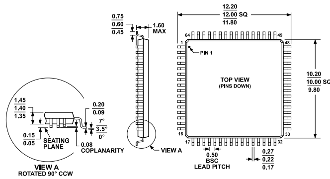
Figure 115. 64-Lead Low Profile Quad Flat Package [LQFP] (ST-64-2) Dimensions shown in millimeters
