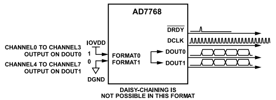
Figure 96. AD7768 FORMATx = 01, Two Data Output Pins
