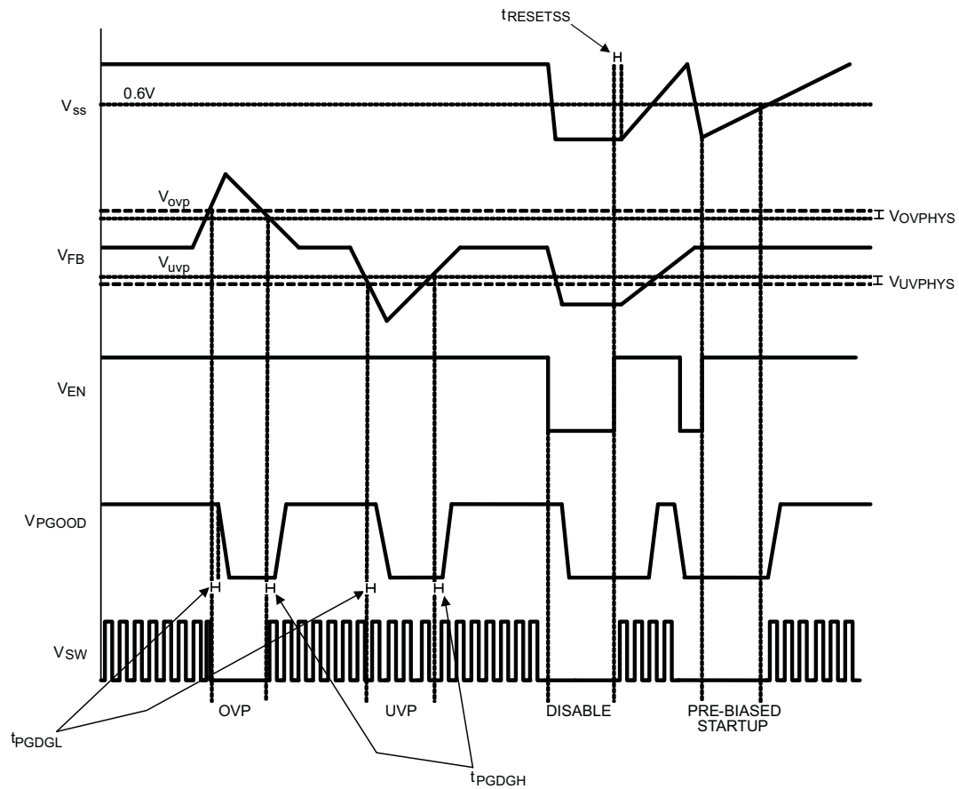
Figure 21. PGGOOD Conditions
