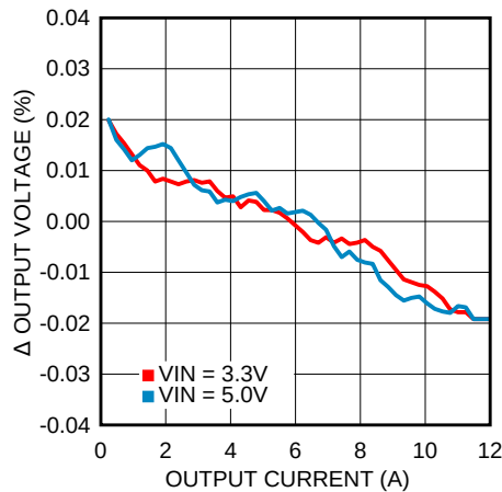
Figure 32. Load Regulation
