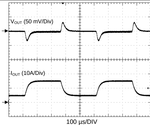
Figure 34. Load Transient Response
