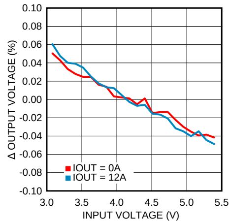
Figure 33. Line Regulation
