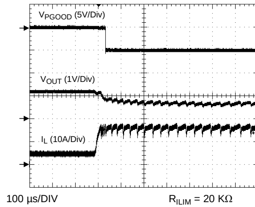
Figure 19. Output Overcurrent Condition
