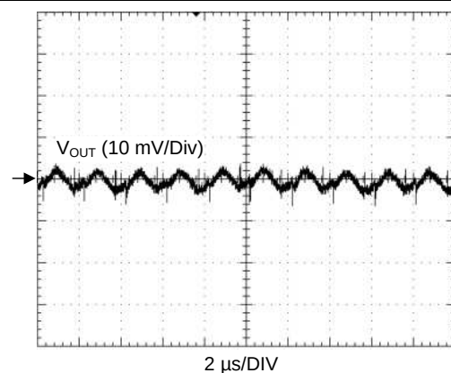
Figure 35. Output Voltage Ripple (IOUT = 15 A)
