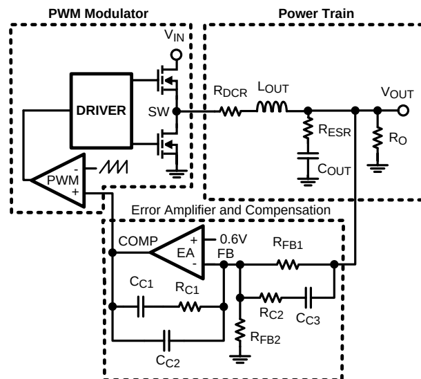
Figure 28. Loop Diagram
