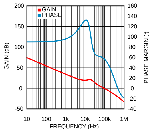
Figure 31. Loop Response
