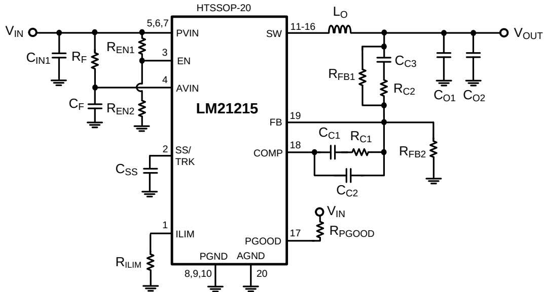
Figure 36. Typical Application Schematic 2
