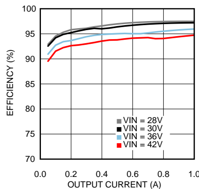
Figure 47. Efficiency V OUT = 24 V, T A = 25°C
