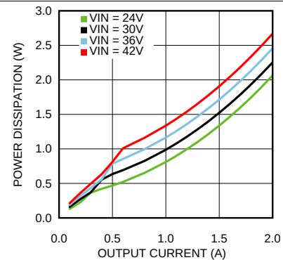
Figure 16. Power Dissipation V_{OUT} = 12\text{ V} T = 85^\circ\text{C}
