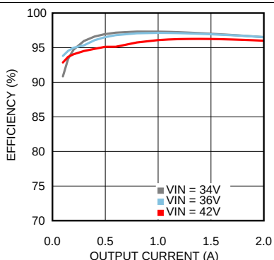
Figure 21. Efficiency V_{OUT} = 24\text{ V} T_A = 85^\circ\text{C}
