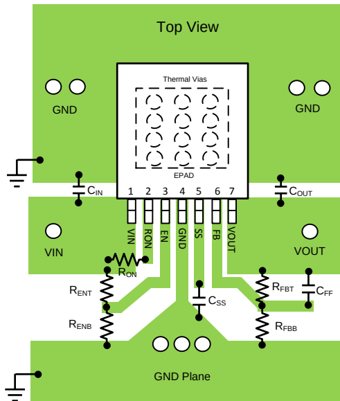
Figure 52. PCB Layout
