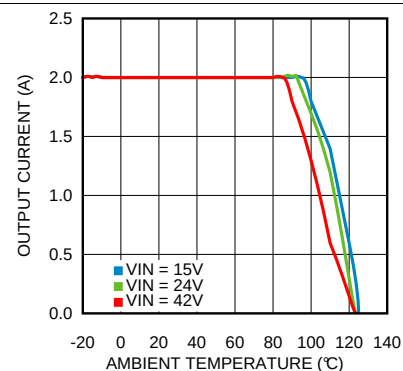
Figure 48. Thermal Derating V_{OUT} = 12 V , R_{\theta JA} = 16^{\circ}C/W
