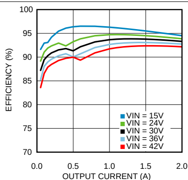
Figure 47. Efficiency V_{OUT} = 12 V
