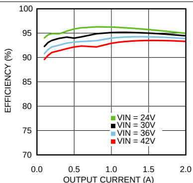
Figure 19. Efficiency V_{OUT} = 18\text{ V} T_A = 85^\circ\text{C}
