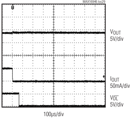
OPEN-LOAD FAULT ( V_{OUT} = 8.5V , I_{OUT} = 50mA )
