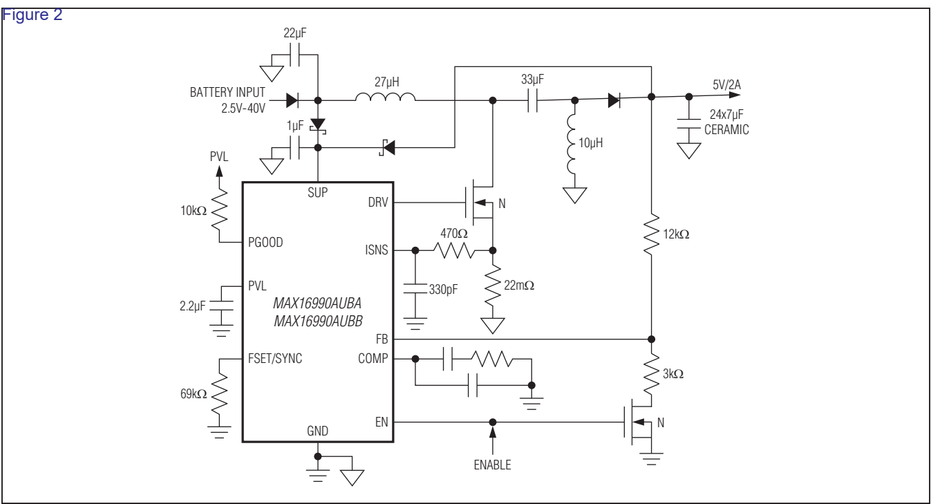
Figure 2. SEPIC Bootstrapped 400kHz Application with Low Operating Voltage
