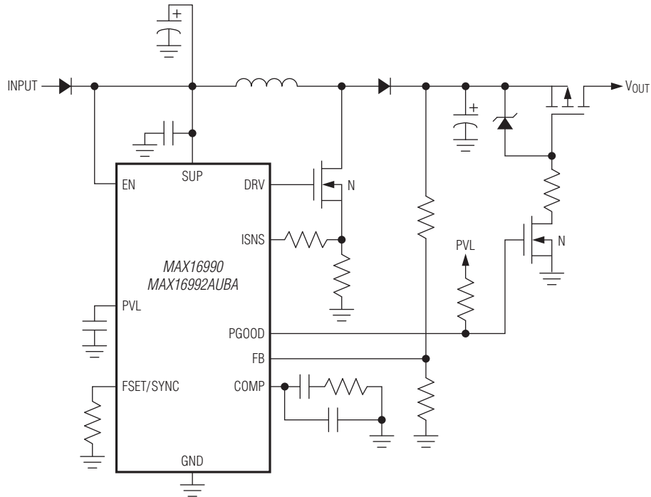
Figure 1. Application with Output Short-Circuit Protection
