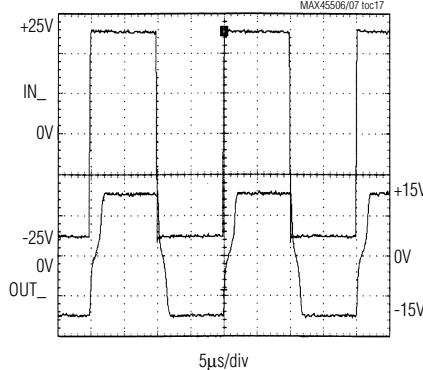
±25V OVERVOLTAGE INPUT WITH THE OUTPUT CLAMPED AT ±15V
