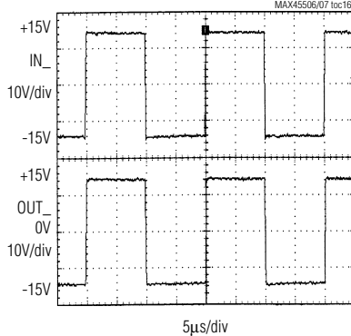
FAULT-FREE RAIL-TO-RAIL SIGNAL HANDLING WITH ±15V SUPPLIES
