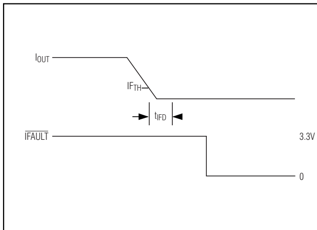
Figure 1. \overline{FAULT} Delay
