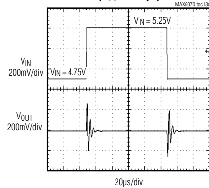
MAX6070_41 LINE TRANSIENT (C OUT = 0.1µF)
