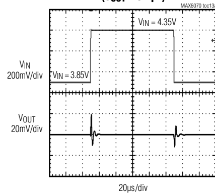
MAX6070_12 LINE TRANSIENT (C OUT = 0.1µF)
