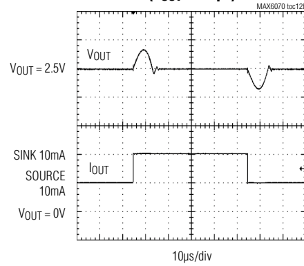
MAX6071_25 ±10mA LOAD TRANSIENT (C OUT = 0.1µF)
