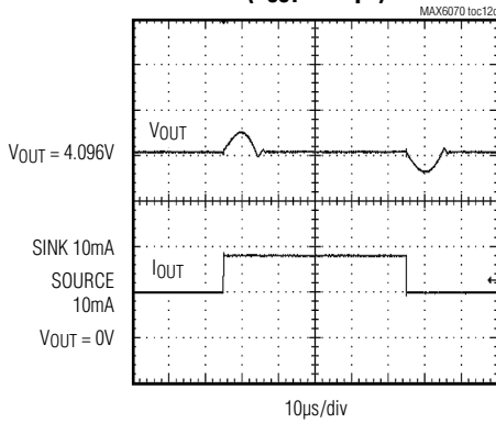
MAX6071_41 ±10mA LOAD TRANSIENT (C OUT = 0.1µF)
