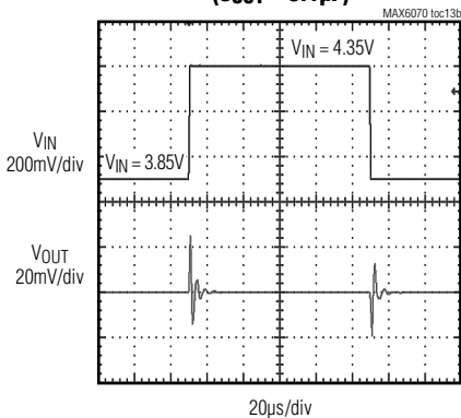
MAX6070_25 LINE TRANSIENT (C OUT = 0.1µF)
