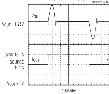
MAX6071_12 ±10mA LOAD TRANSIENT (C OUT = 0.1µF)
