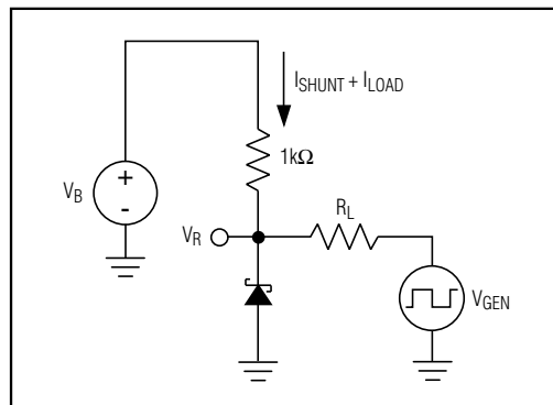
Figure 1. Load-Transient Circuit
