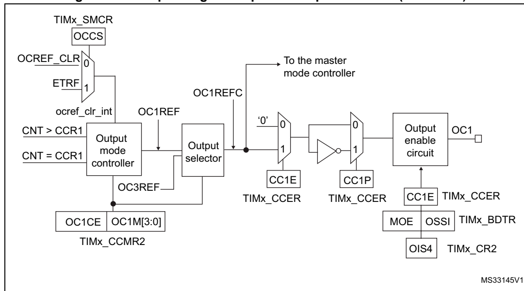
Figure 234. Output stage of Capture/Compare channel (channel 1)
