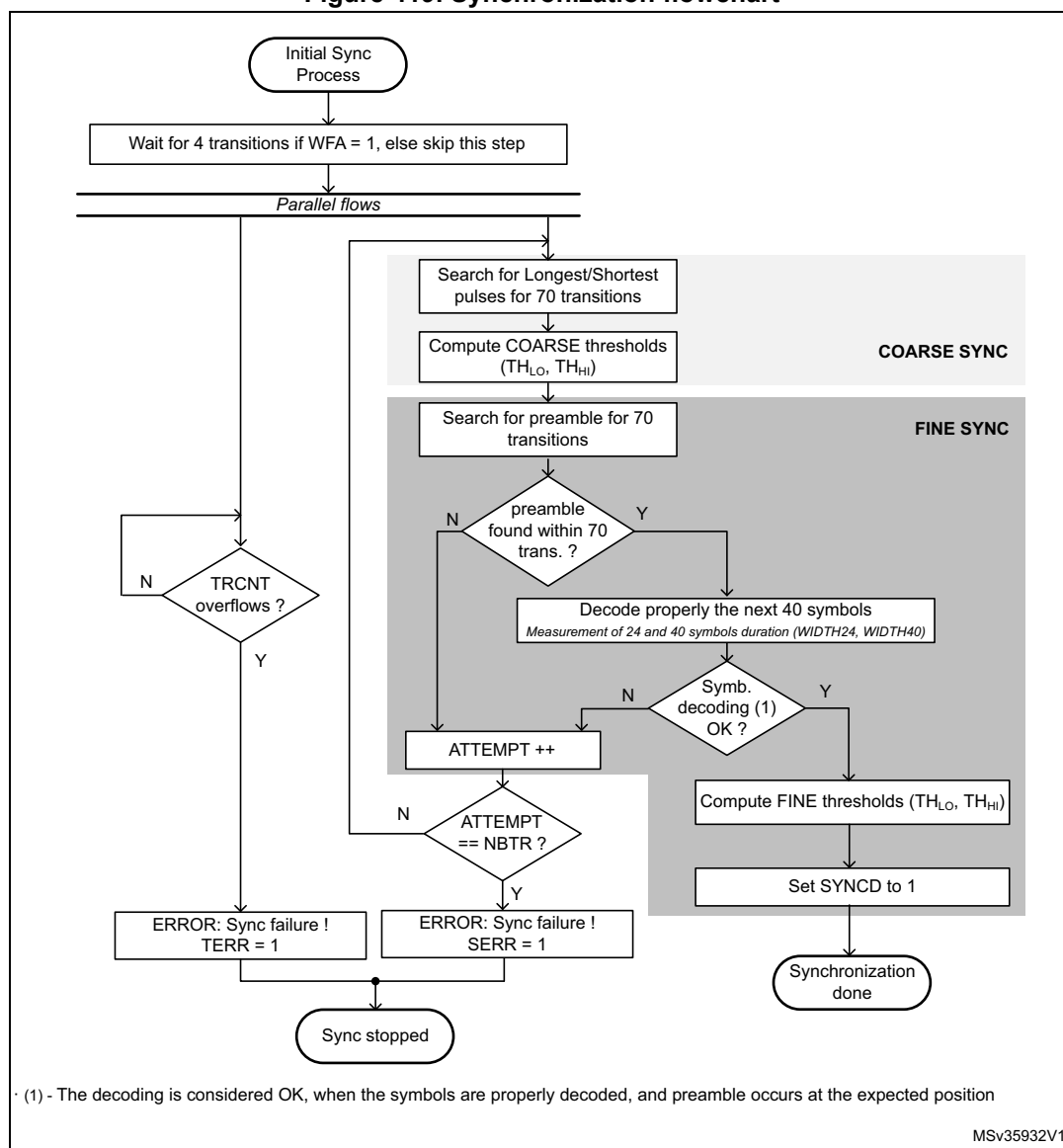
Figure 419. Synchronization flowchart
