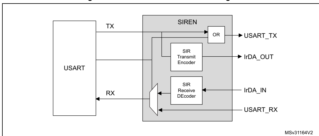
Figure 349. IrDA SIR ENDEC- block diagram
