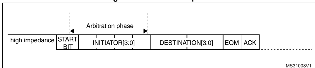
Figure 530. Arbitration phase
