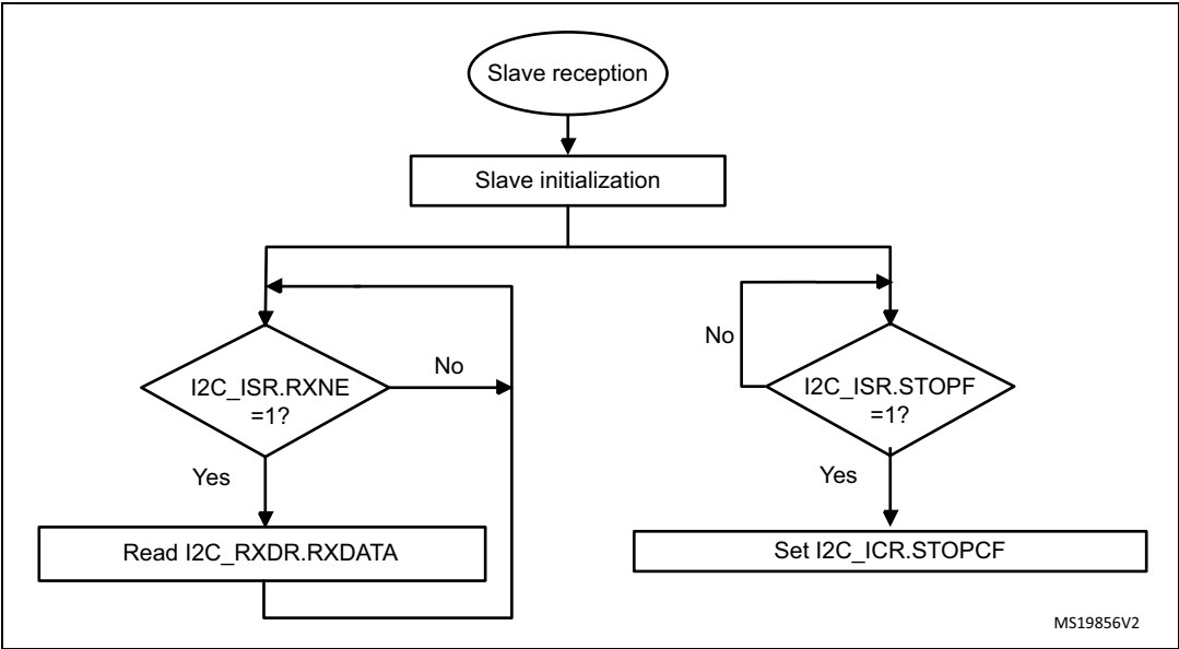
Figure 313. Transfer sequence flowchart for slave receiver with NOSTRETCH=1
