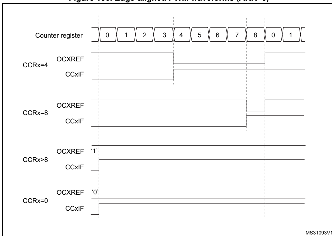
Figure 183. Edge-aligned PWM waveforms (ARR=8)
