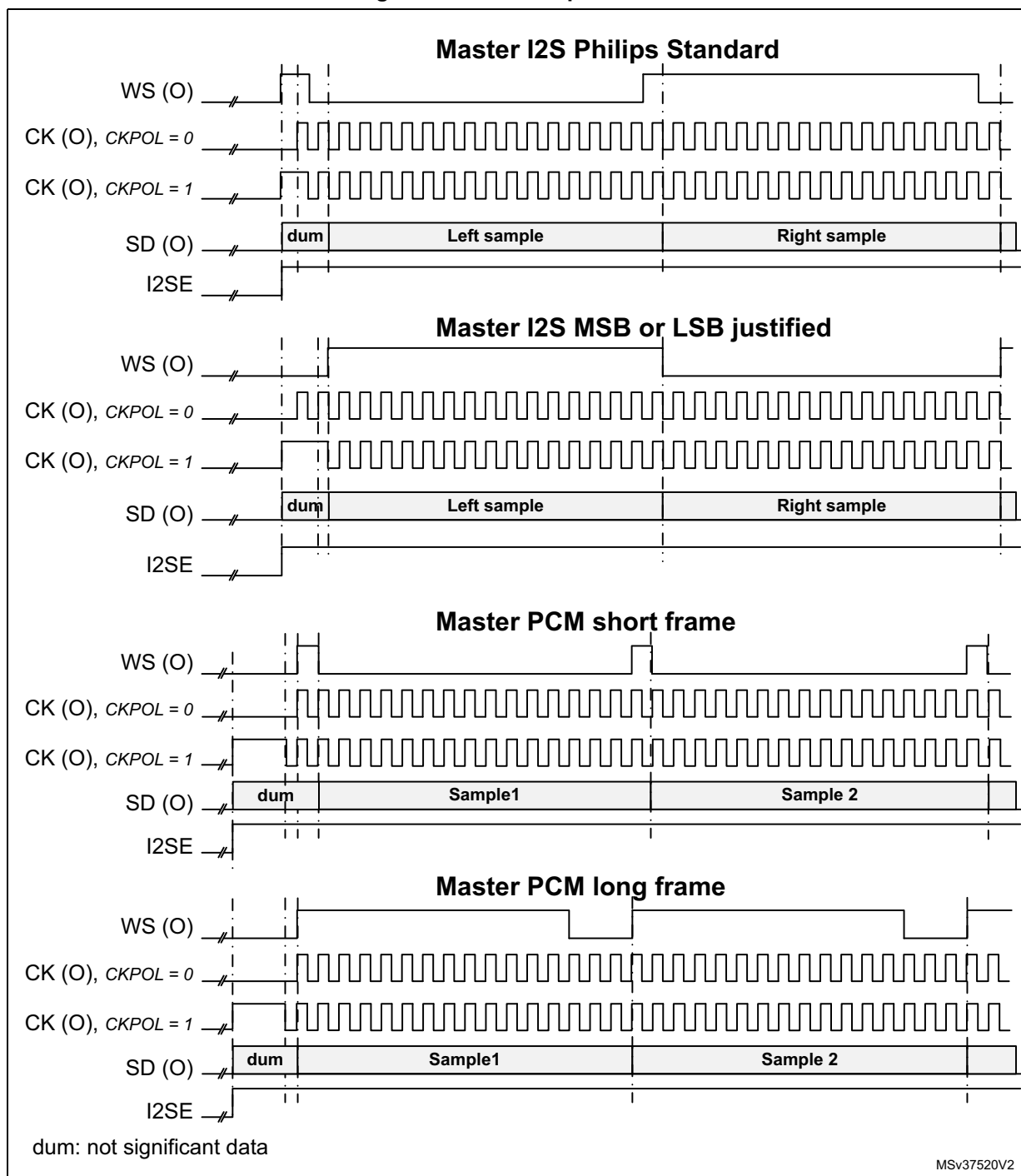
Figure 392. Start sequence in master mode
