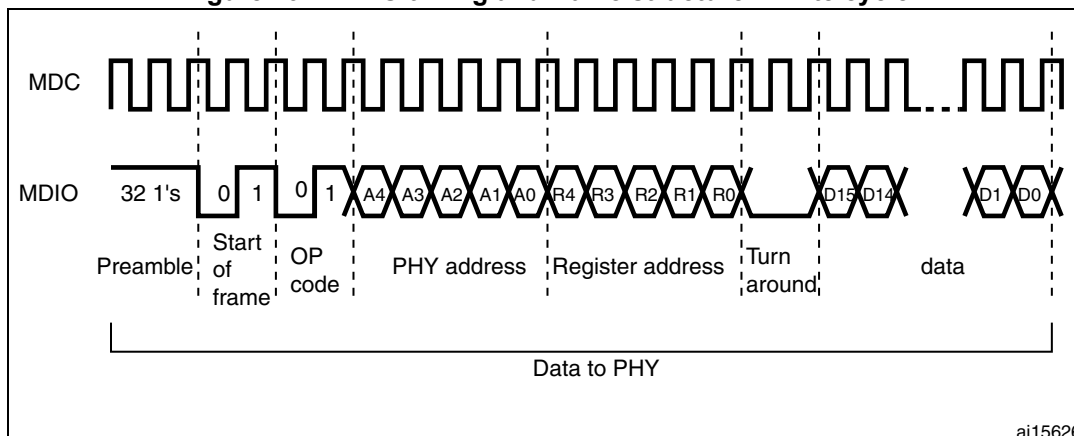
Figure 491. MDIO timing and frame structure - Write cycle
