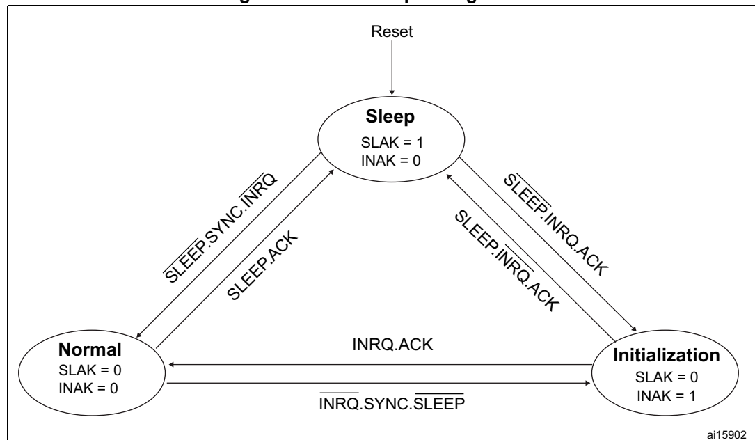
Figure 443. bxCAN operating modes
