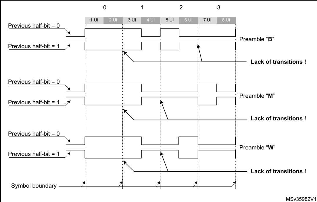
Figure 414. S/PDIF Preambles
